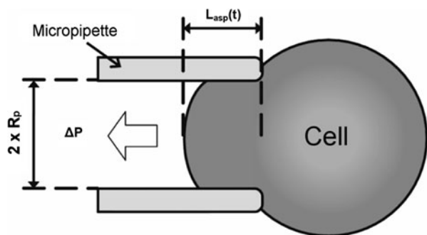
FIGURE 4. Cell aspiration schematic indicating key parameters in the elastic half space analytical model.
