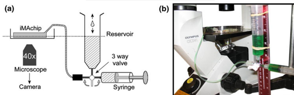
FIGURE 2. (a) Schematic diagram of pressure system. The three-way valve is used to switch between applying large, uncontrolled pressures via the syringe, and applying small well controlled pressures via the liquid column in the reservoir. Adding or removing liquid to the reservoir changes the pressure applied. (b) Experimental setup for iMAchip peripherals (green dye used for this demonstration).
