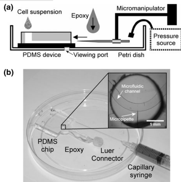
FIGURE 1. (a) Schematic side-view of the device, demonstrating fabrication and operation of the iMAchip device. The micropipette is manipulated into the PDMS device, and epoxied into place on the Petri dish. The slip-mounted micromanipulator fitting is withdrawn, and the device is primed, loaded with a cell suspension, and connected to a pressure source for cell aspiration. (b) Fabricated iMAchip system (pictured with capillary syringe used to prime the micropipette with deionized water prior to use; colored dye used for clarity).
