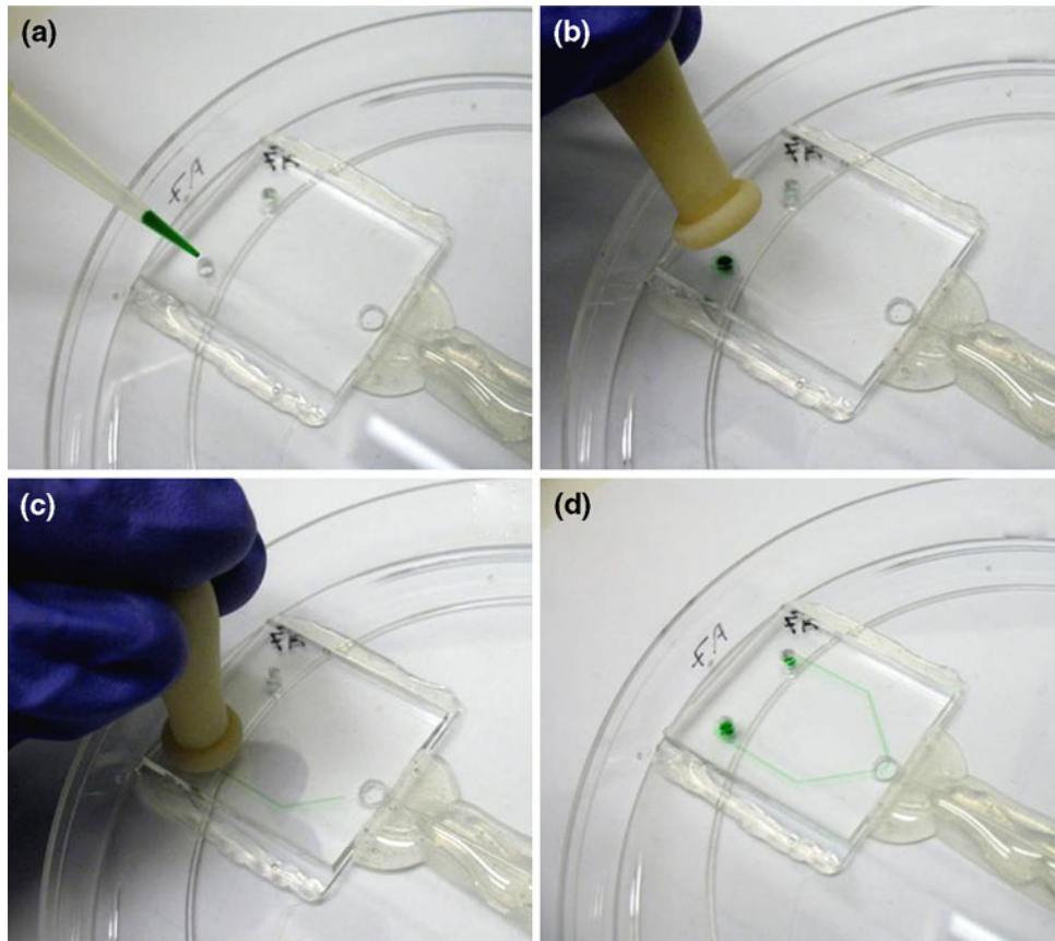
FIGURE 3. Loading cell samples (green dye used for clarity) into the iMAchip devices. (a) Cell suspension is pipetted into the microchannel access port. (b) A Pasteur pipette bulb is placed over the port and (c) gently squeezed, (d) driving fluid flow through the channel.
