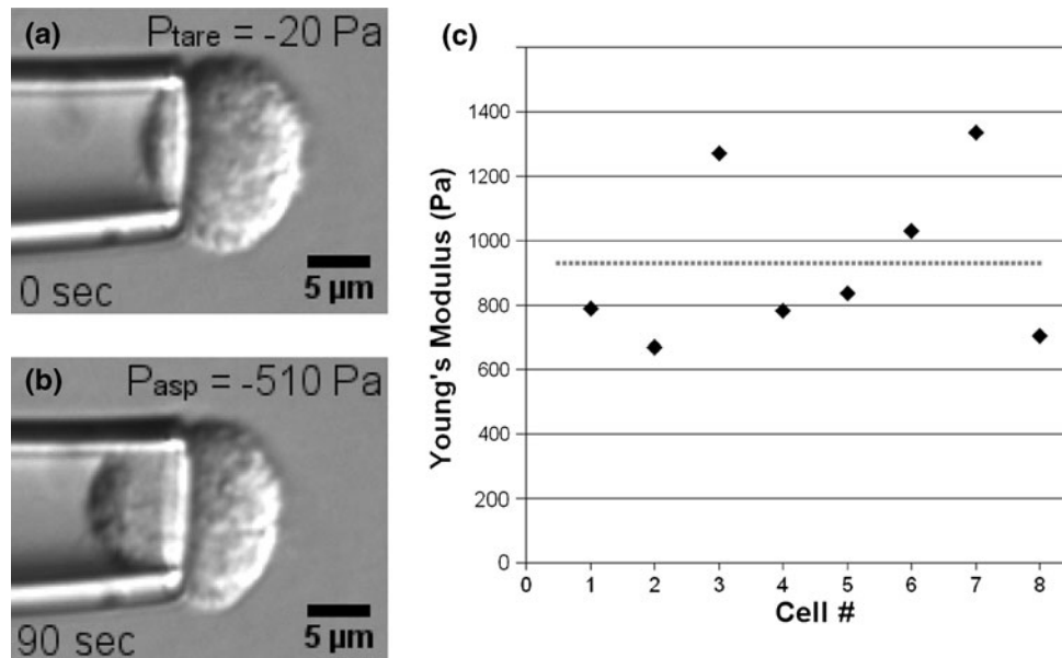
FIGURE 5. (a, b) Sample images of cells being aspirated at a tare pressure and at a higher aspiration pressure. (c) Young's modulus for eight individual single cells, calculated using the elastic half-space model. Mean modulus value represented as a dotted line.
