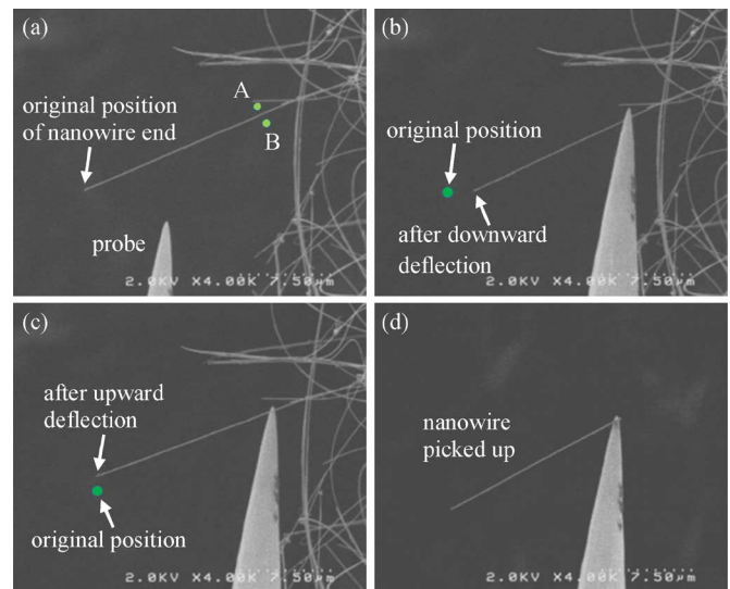
Fig. 4. Nanowire pick-up. (a) A probe is brought close to a nanowire. (b) The probe descends and contacts the nanowire and ascends to contact it. (c) The probe descends underneath the nanowire and ascends to contact it. (d) The nanowire is EBID-soldered to the probe and picked up.
