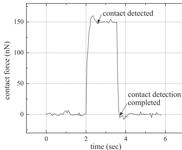
Fig. 16. Contact force monitoring for reliable contact detection.
