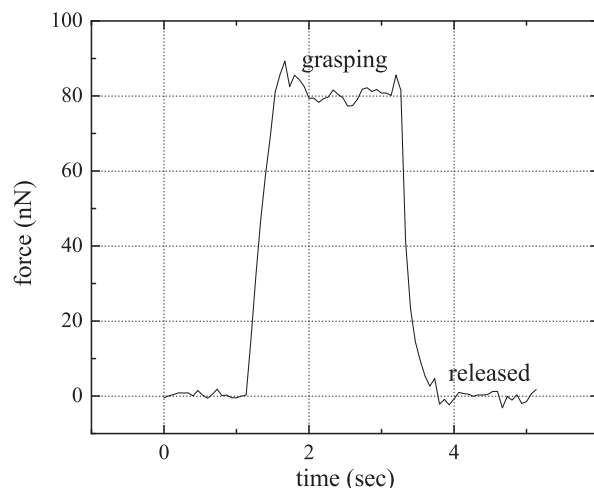
Fig. 17. Grasping force profile during micrograsping and releasing of a cell.
