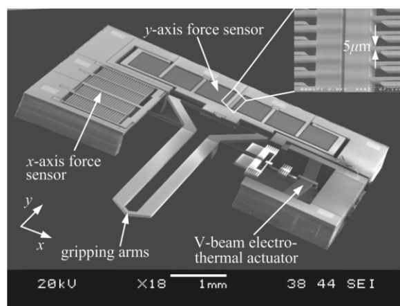
Fig. 12. MEMS-based microgripper with integrated two-axis capacitive force sensors.
